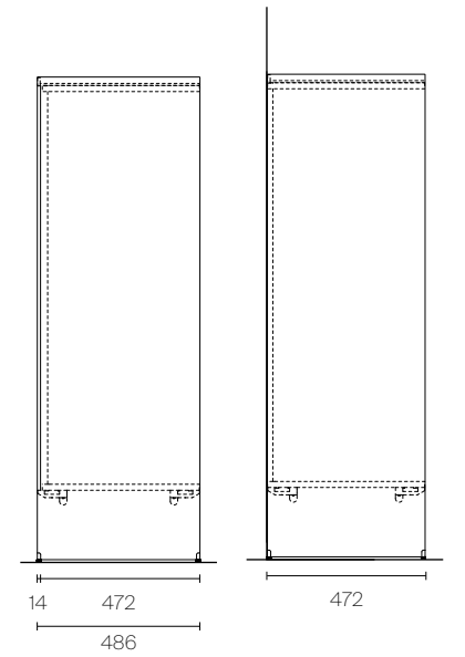
Double sided composition raised version H 240 Wall compositions raised version H 240
