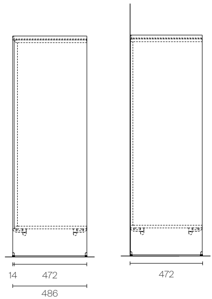
Double sided composition raised version H 186 Wall compositions raised version H 186
