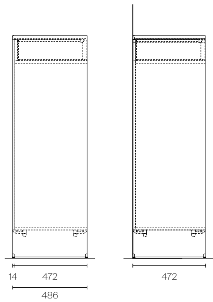
Double sided composition raised version H 186 with open compartment Wall compositions raised version H 186 with open compartment
