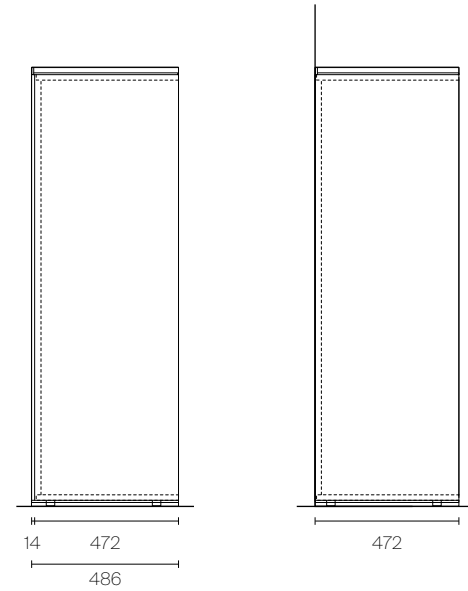
Double sided composition with foot H 20
