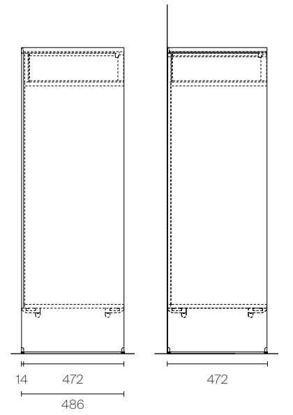
Double sided composition raised version H 240 with open compartment Wall compositions raised version H 240 with open compartment
