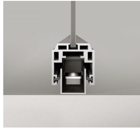
Floor guide profile for side installation
