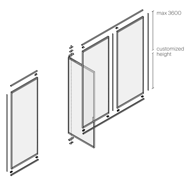
Fixed panels and bi-directional door - side installation
