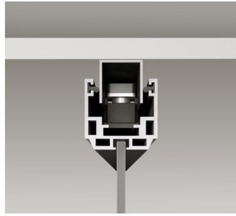
Ceiling profile
