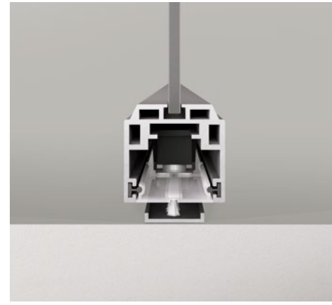
Floor guide profile for front installation
