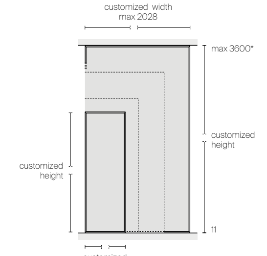
Air system pure
