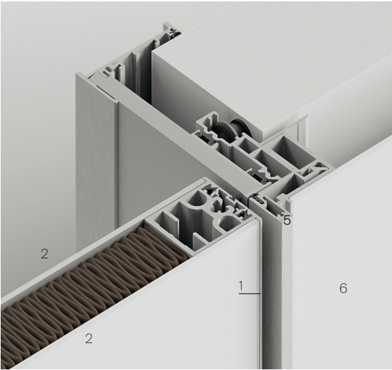
BI-DIRECTIONAL DOOR COMBINED WITH MODULOR PANELLING
