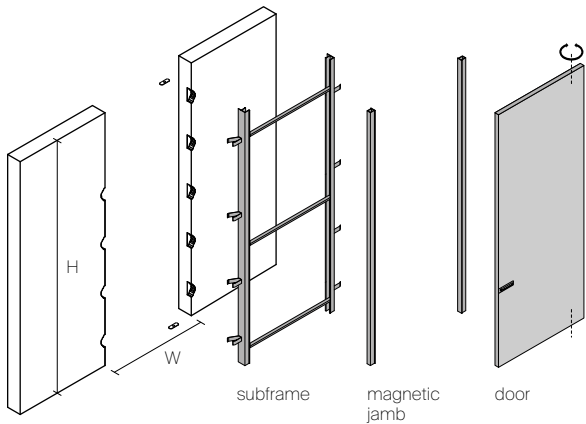
Bi-directional door with jamb and magnetic locking profile
