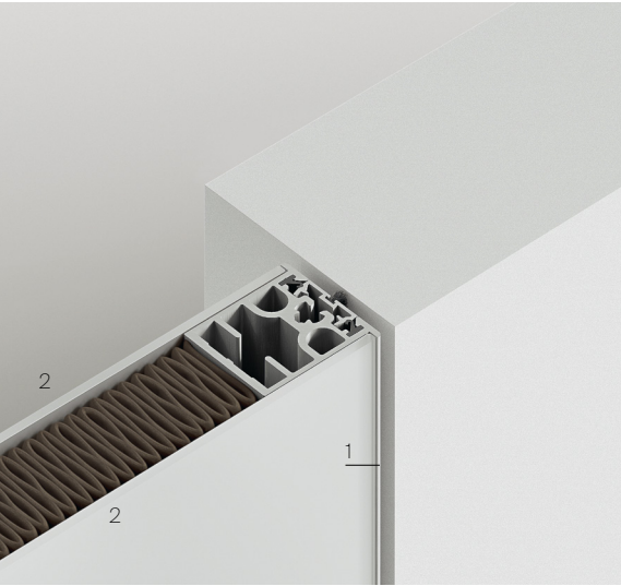
BI-DIRECTIONAL DOOR WITHOUT JAMB
