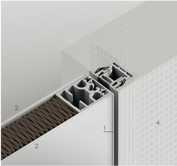
BI-DIRECTIONAL DOOR WITH JAMB AND MAGNETIC LOCKING PROFILE
