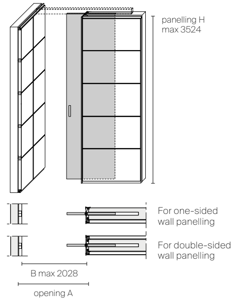
Full-height single pocket door against Modulo panel
