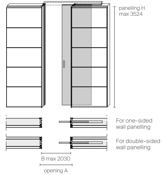
Full-height single pocket door against Modulo panel
