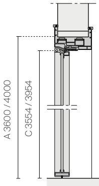
Wall flush swing door with fanlight
