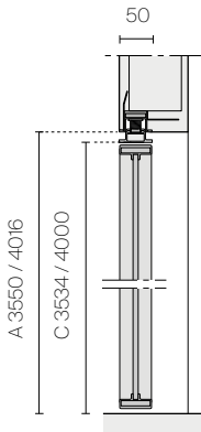
Wall flush swing door with fanlight
