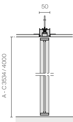
Ceiling flush swing door with fanlight
