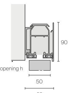
Single rail Maxi
