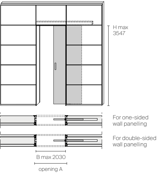
Full-height single pocket door
