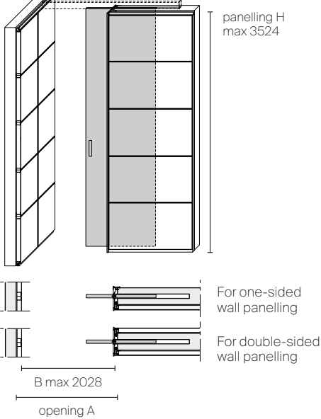
Full-height single pocket door against Modulor panel
