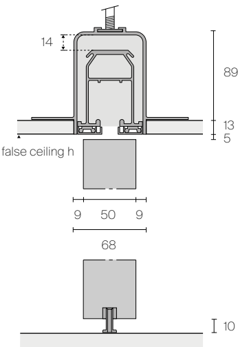
Single built-in rail Maxi
