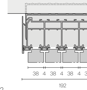
Four ways rail
