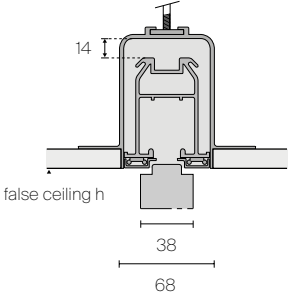
Double rail
