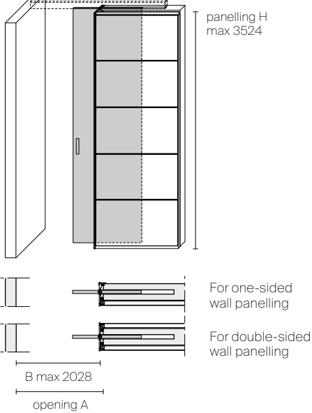
Full-height single pocket door against wall
