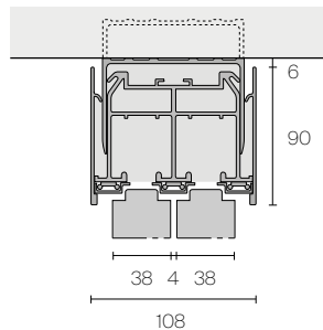
Three ways rail
