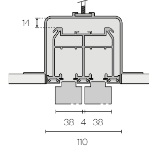
Three ways rail
