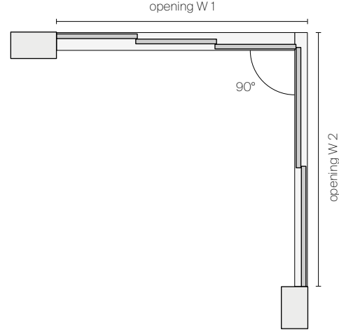
Double and 4 ways rail in the opening
