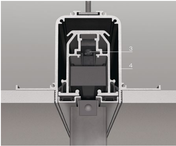
Built-in rail
