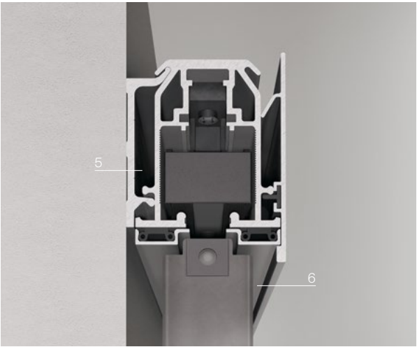
Wall rail
