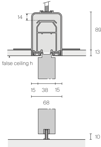
Single built-in rail
