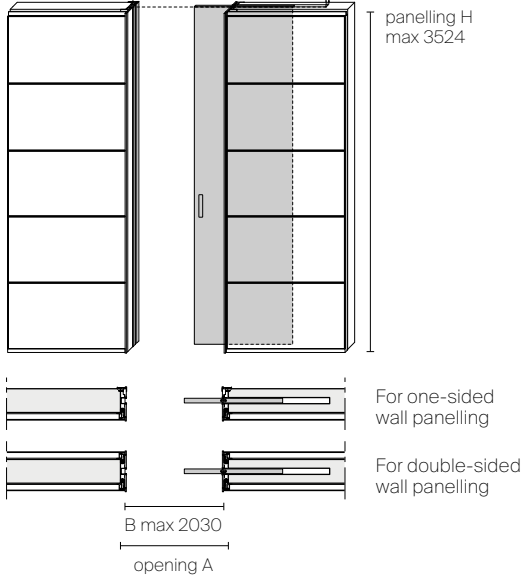
Full-height single pocket door against Modulor panel
