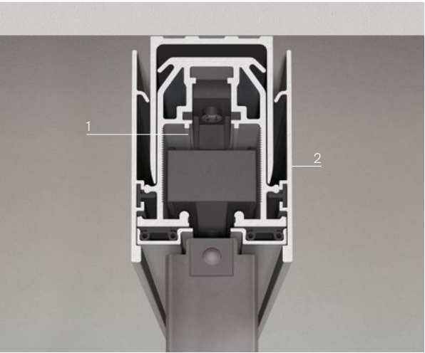
Ceiling rail
