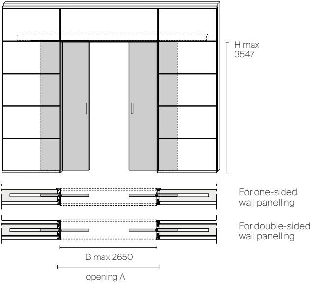
Full-height double pocket door
