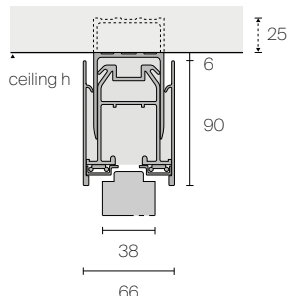
Double rail
