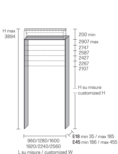
passaggio completo E18 complete passage E18 estensibile da mm 35 a mm 185 extensible from mm 35 to mm 185
