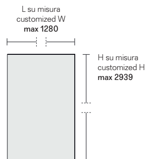
schienale in vetro glass back panel
