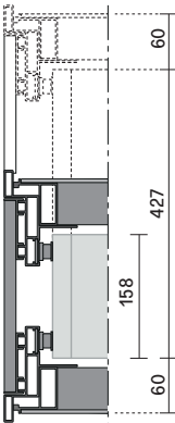
passaggio completo E42 complete passage E42 estensibile da mm 158 a mm 427 extensible from mm 158 to mm 427
