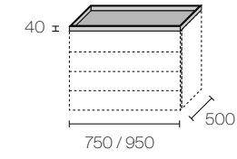
Suspended melamine drawer unit
