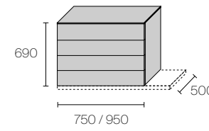
Melamine drawer unit on wheels with four drawers
