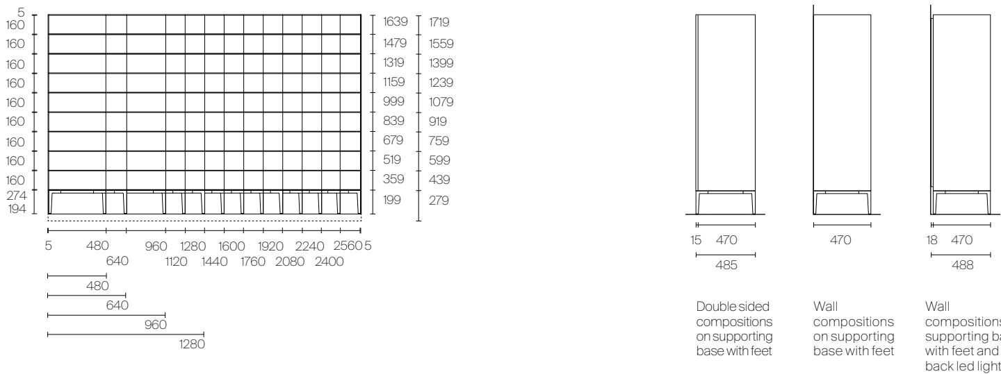
Self bold 26 - modularity D 470
