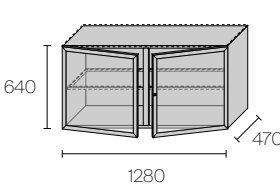
Cabinet with transparent glass hinged doors equipped with lock
