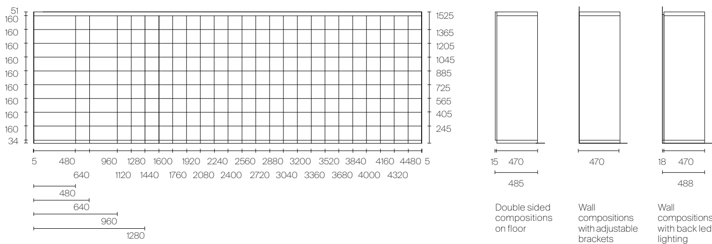
Self bold 51 - modularity D 470
