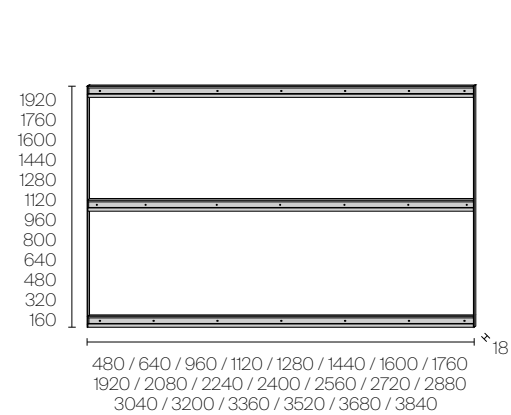
Frame for backlitged suspended cabinets with lighting system and additional crosspiece for brackets for stacked suspended units
