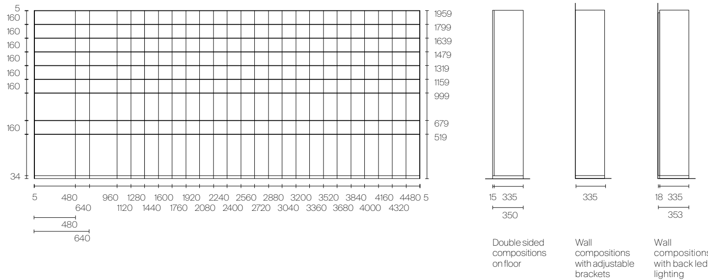
Self up - modularity D 335
