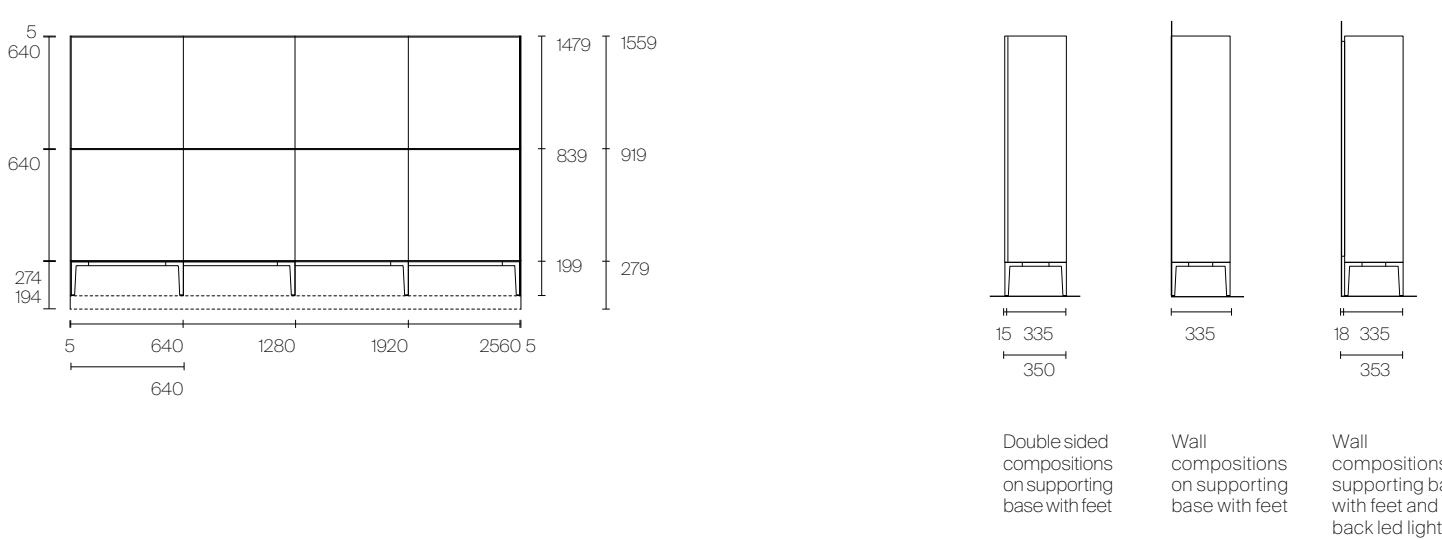
Self bold 51 - modularity D 470
