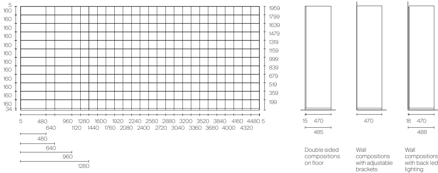
Self up - modularity D 470
