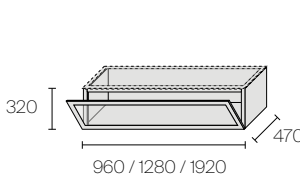
Cabinet with glass flap door
