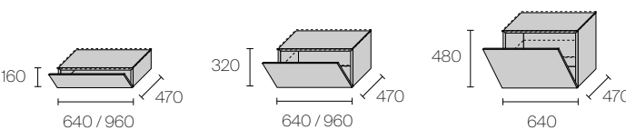
Hinged door units
