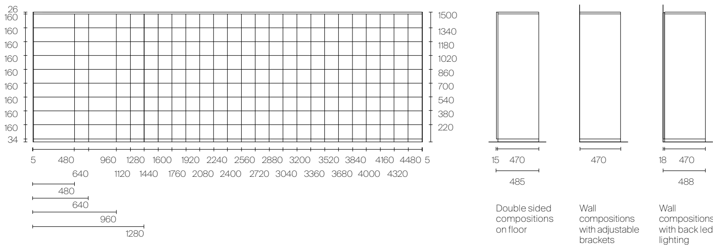
Self bold 26 - modularity D 470
