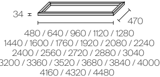
Glass or Litech top
