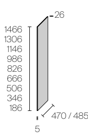
Lower or upper single led lighting
