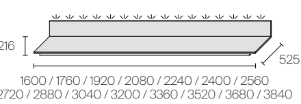
Writing desk version without side panels. Optional led lighting
