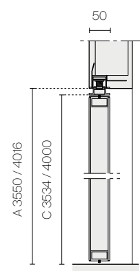
Wall flush swing door with fanlight
